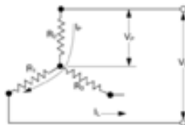
3-Phase Wye (Balanced Load)
